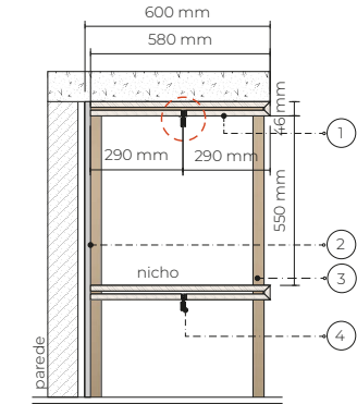
CORTE VERTICAL
