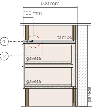
CORTE VERTICAL
