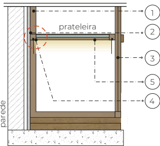
CORTE VERTICAL
