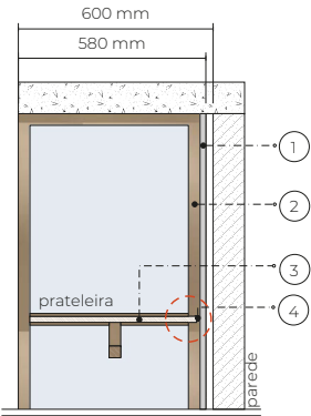
CORTE VERTICAL
