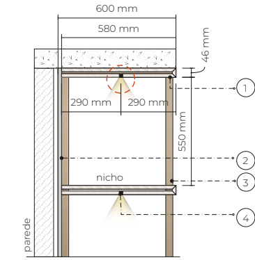
CORTE VERTICAL
