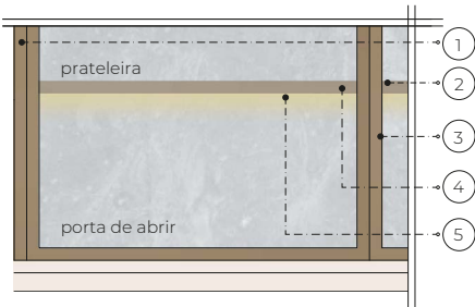
VISTA FRONTAL
