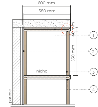
CORTE VERTICAL
