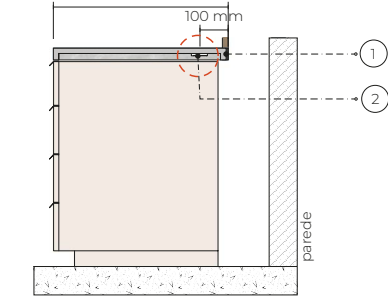
CORTE VERTICAL
