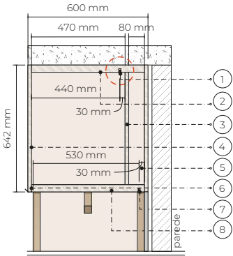
CORTE VERTICAL
