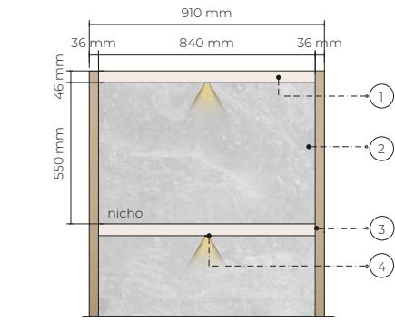
VISTA FRONTAL
