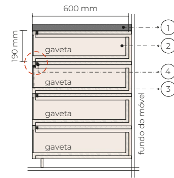
CORTE VERTICAL
